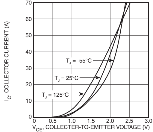
FIGURE 2, Output Characteristics ( V_{GE} = 10V )
