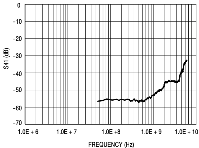
Figure 2. Analog Crosstalk Curve (S41 Measurement)
