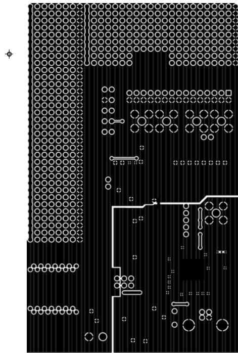
Figure 9. AD7795 Evaluation Board Solder Side Artwork
