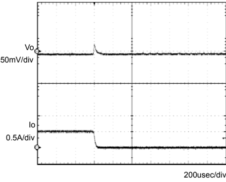
Fig.2 Transient Response (0.5→0A) C_o=1\mu\text{F}
