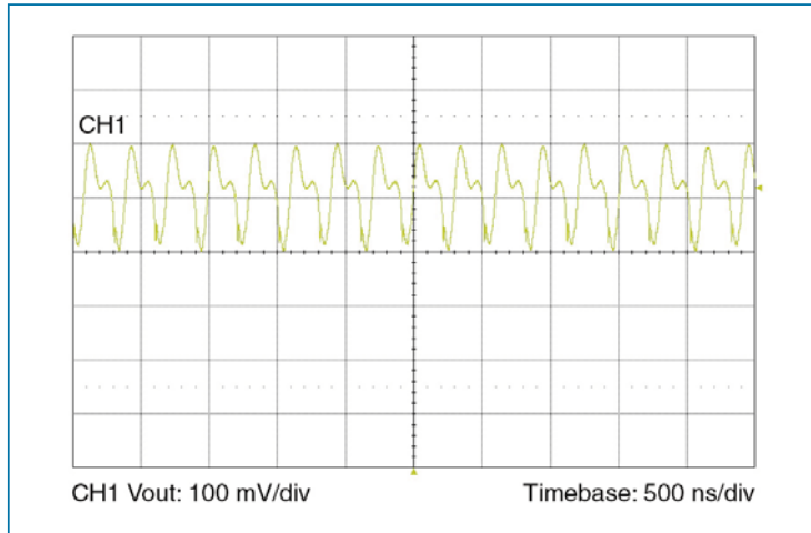
Figure 7 — Output voltage ripple at full load and 352 Vin without any external bypass capacitor.
