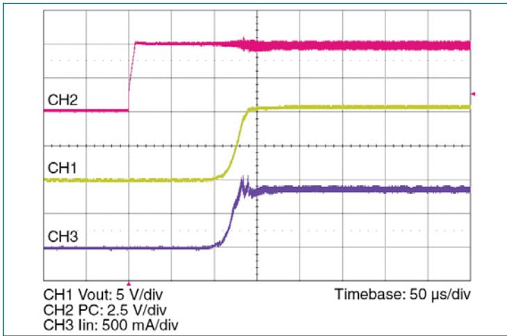
Figure 1 — Inrush transient current at full load and 352 Vin with PC enabled
