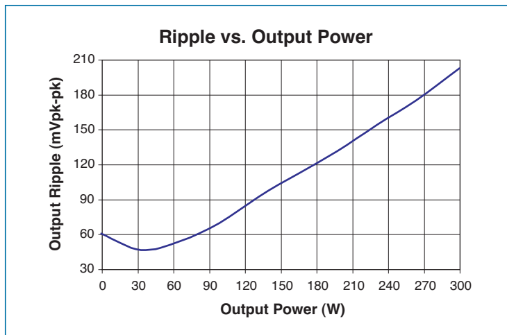
Figure 9 — Output voltage ripple vs. output power at 352 Vin without any external bypass capacitor.
