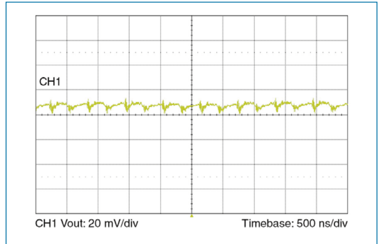
Figure 8 — Output voltage ripple at full load and 352 Vin with 10 \mu\text{F} ceramic external bypass capacitor and 20 nH of distribution inductance.
