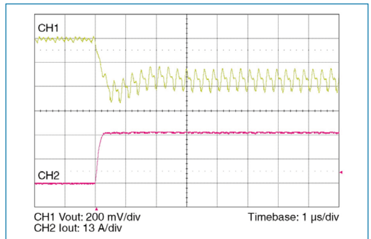
Figure 10 — 0-27.3 A load step with 2 \mu\text{F} input capacitor and no output capacitor.
