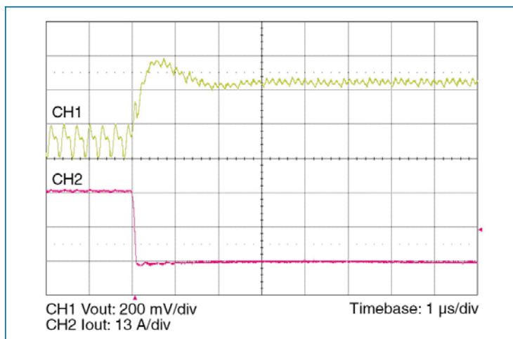
Figure 11 — 27.3-0 A load step with 2 \mu\text{F} input capacitor and no output capacitor.
