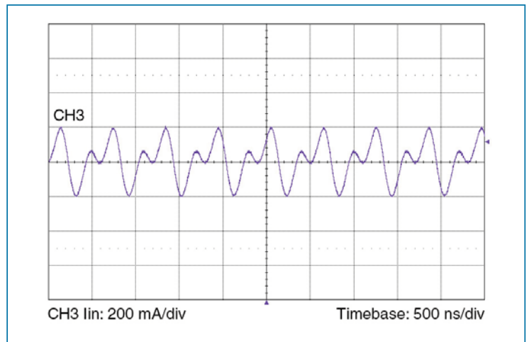
Figure 4 — Input reflected ripple current at full load and 352 Vin
