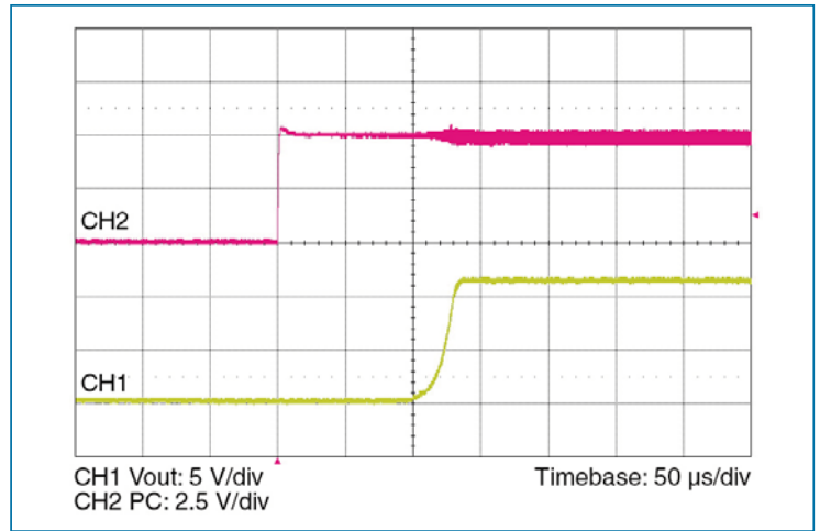
Figure 2 — Output voltage turn-on waveform with PC enabled at full load and 352 Vin
