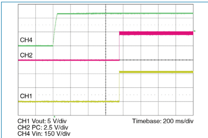
Figure 3 — Output voltage turn-on waveform with input turn-on at full load and 352 Vin
