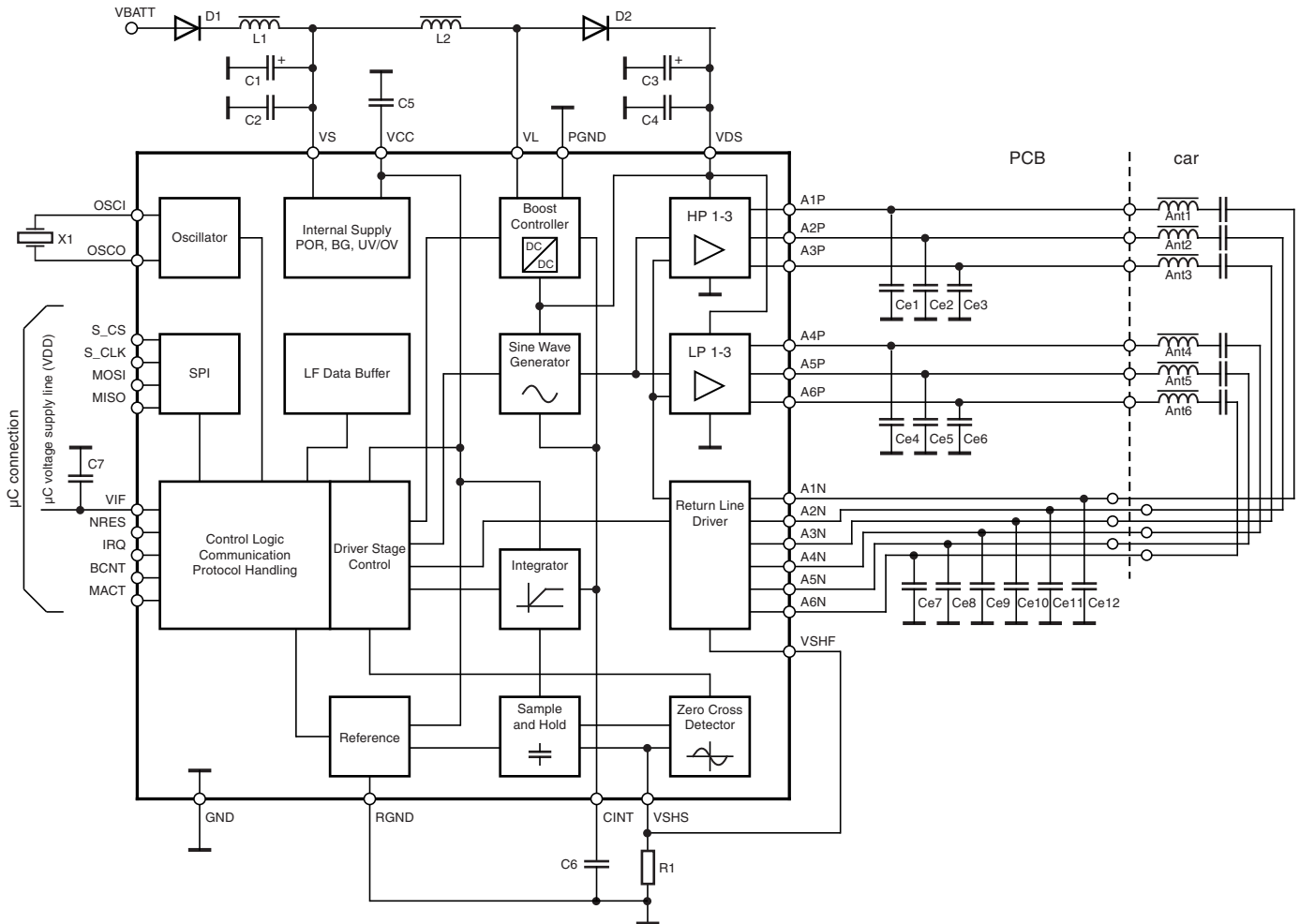
Figure 4-1. Application Schematic for ATA5279N
