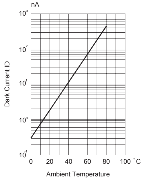
Figure 4. DARK CURRENT VS. AMBIENT TEMPERATURE VR=10 , E_e=0\text{mW/cm}^2
