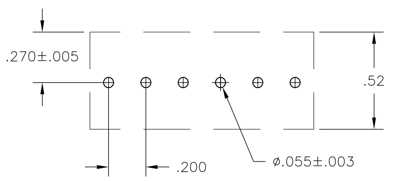
RECOMMENDED BOARD LAYOUT
