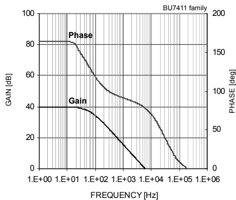
Fig.69 Gain – Frequency
