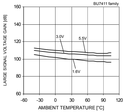
Fig.63 Large Signal Voltage Gain – Ambient Temperature
