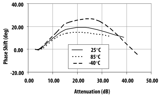
Figure 25. Phase shift vs Attenuation vs Temperature at 1900MHz
