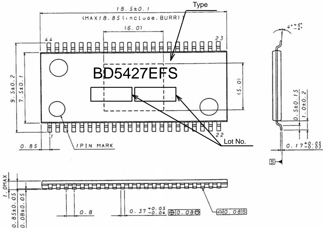
Fig. 23 Outer Dimensions and Inscriptions of HTSSOP-A44 Package
