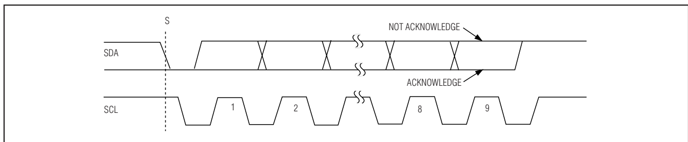
Figure 20. Acknowledge Bits
