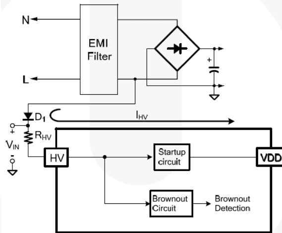
Figure 6. Brownout Circuit
