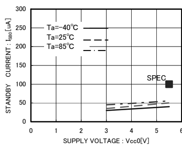
Fig.21 Standby Current I SB0
