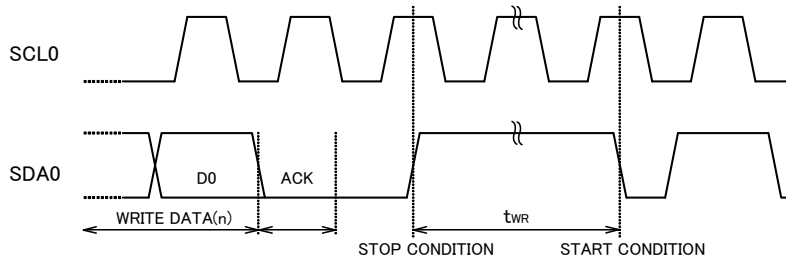
Fig.40 WRITE CYCLE TIMING
