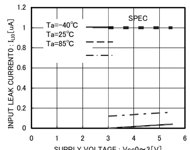
Fig.16 Input Leak Current0 I IL0 (SCL0~3)
