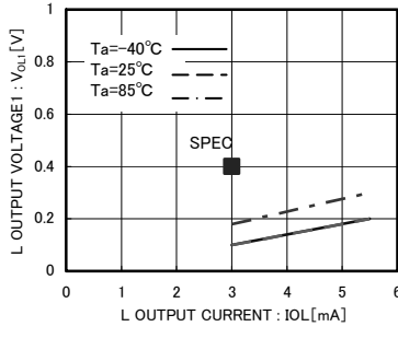
Fig.11 'L' Output Voltage1 V OL1 -I OL (V CC1 =3.0V) (SDA1)
