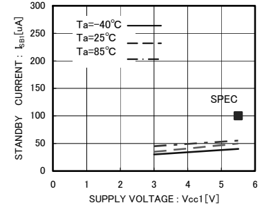
Fig.22 Standby Current I SB1
