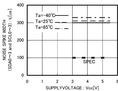
Fig.35 Noise Spike Width t_i (SDA0~3 and SCL0~3)
