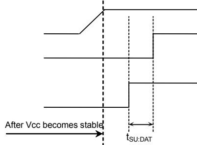
Fig.62 When SCL0~3='L' and SDA0~3='L'
