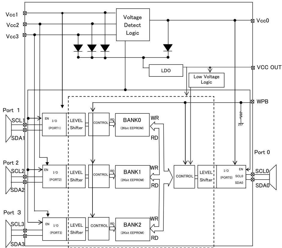
Fig.38 BLOCK DIAGRAM
