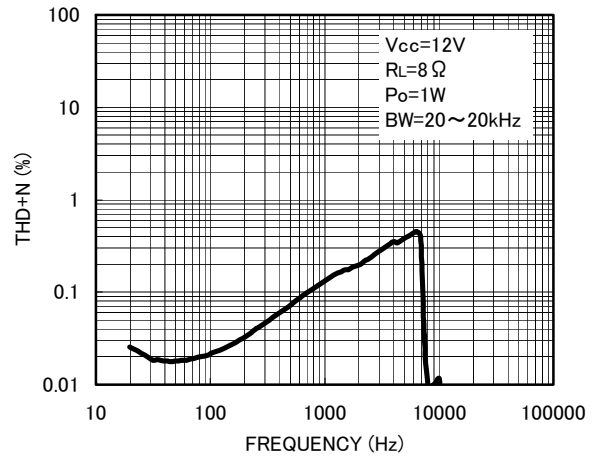
Fig. 2 THD+N - Frequency
