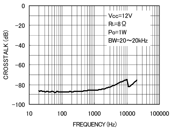
Fig. 4 Crosstalk - Frequency
