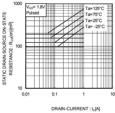
Fig.7 Static Drain-Source On-State Resistance vs. Drain Current(IV)
