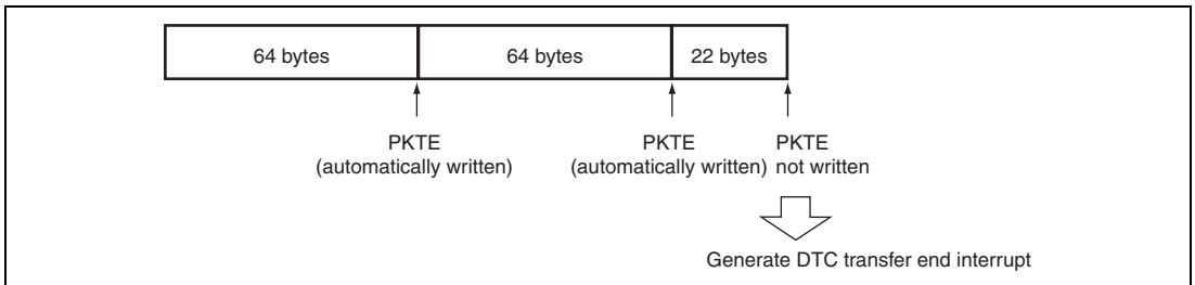
Figure 25.24 EP2 PKTE Operation
