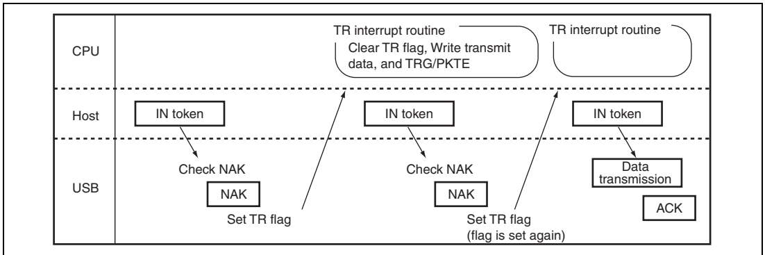
Figure 25.28 Timing for Setting the TR Interrupt Flag
