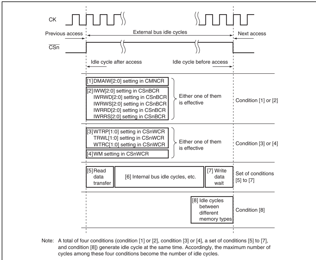
Figure 9.41 Idle Cycle Conditions
