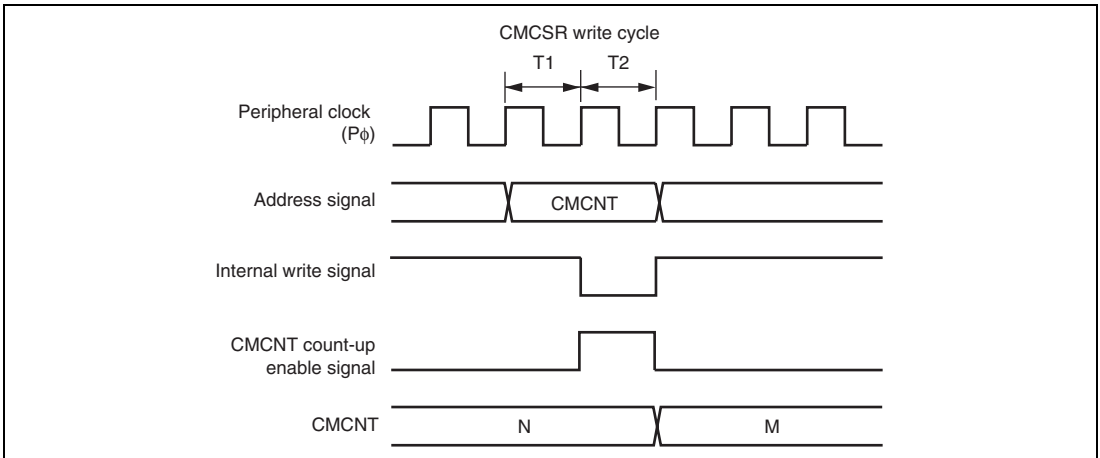
Figure 14.6 Conflict between Word-Write and Count-Up Processes of CMCNT
