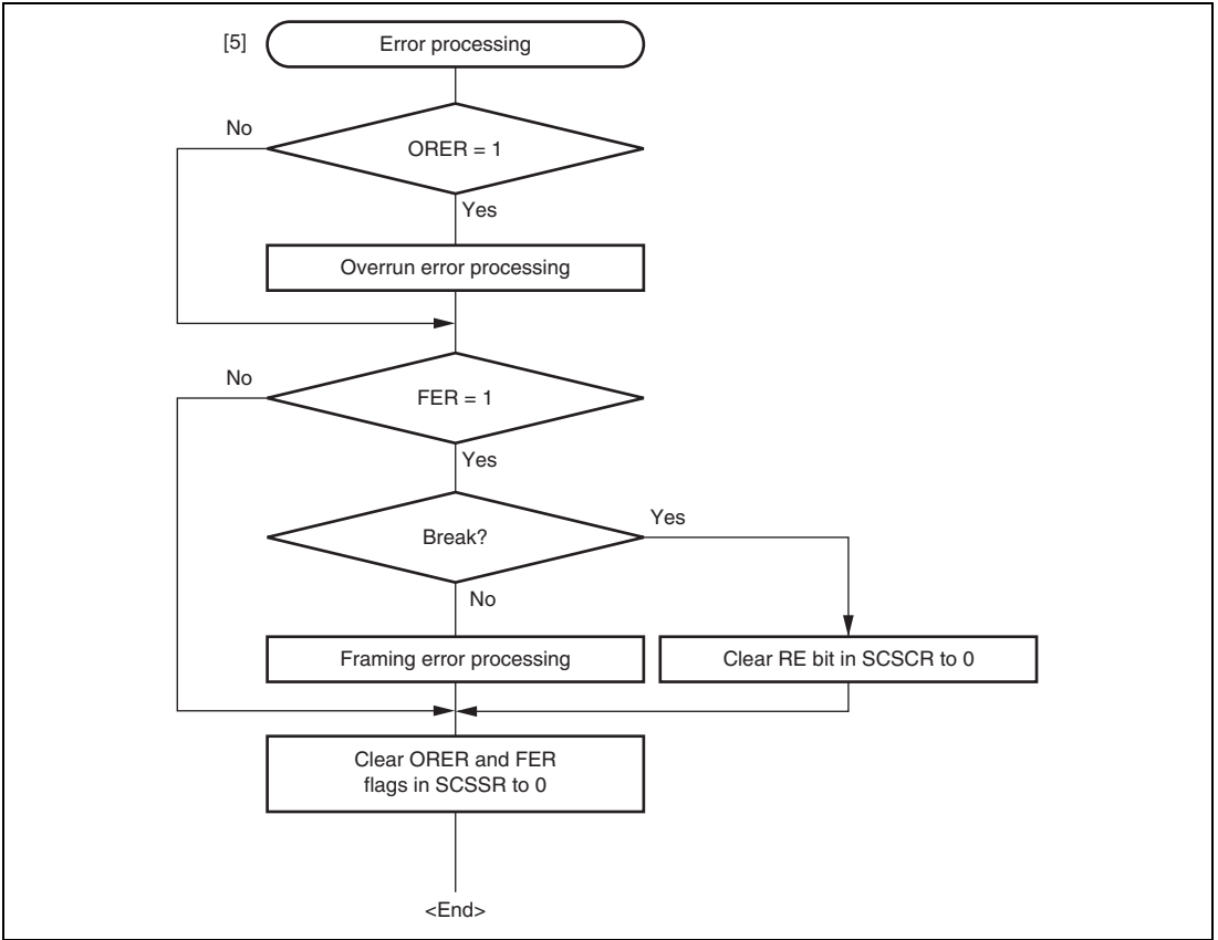
Figure 16.18 Sample Multiprocessor Serial Reception Flowchart (2)
