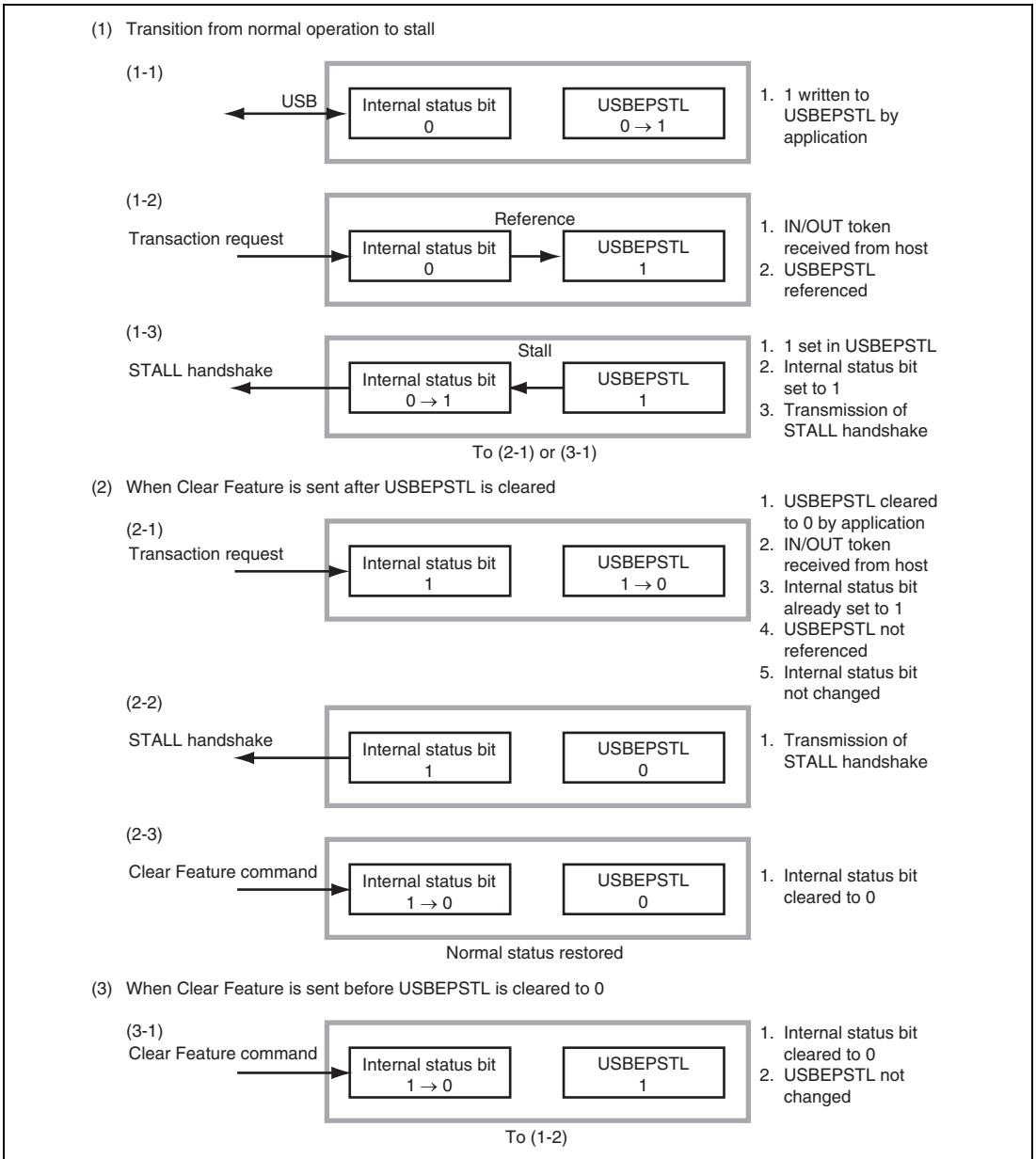
Figure 25.13 Forcible Stall by Application
