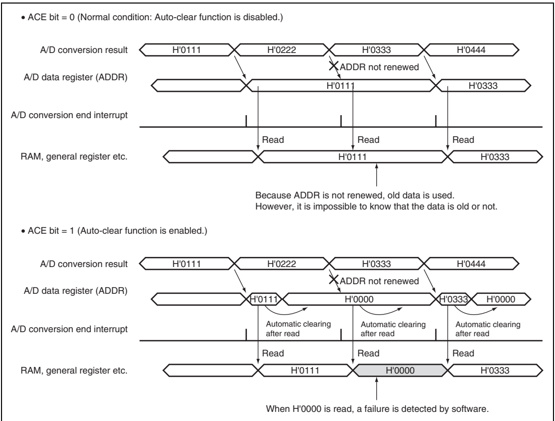
Figure 20.12 Example of When ADDR Auto-clear Function is Disabled (Normal Condition)/Enabled
