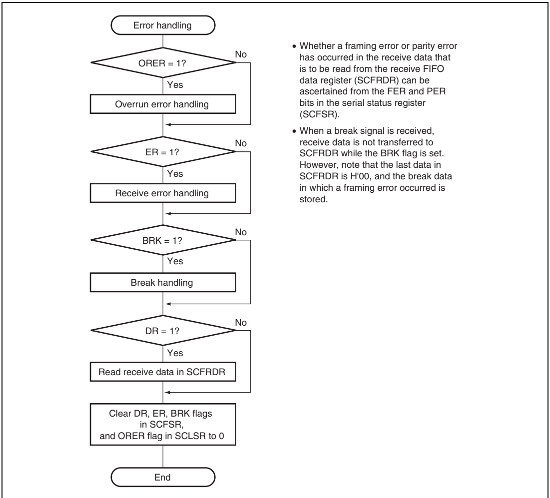
Figure 17.7 Sample Flowchart for Receiving Serial Data (cont)
