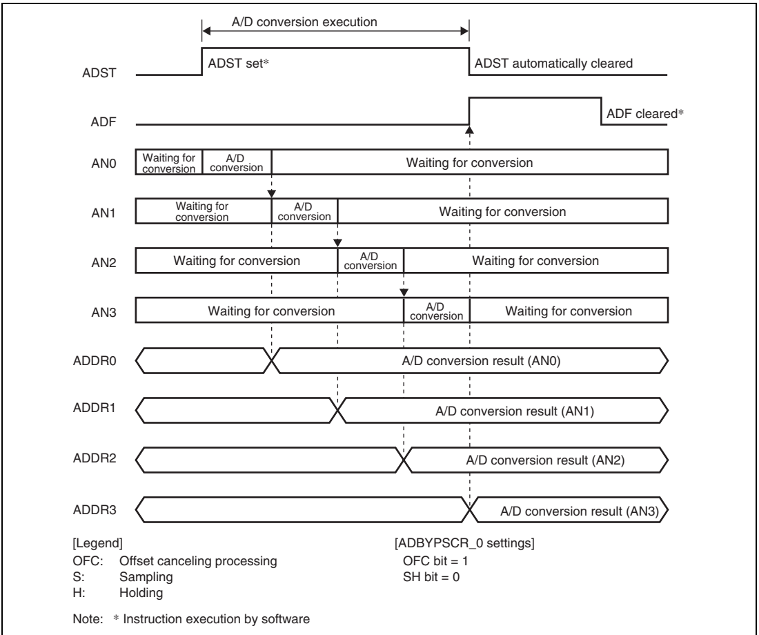
Figure 20.5 Example 4 of A/D_0 Converter Operation (Single-Cycle Scan Mode, Sample-and-Hold Circuit Disabled, and Offset Canceling Circuit Disabled)
