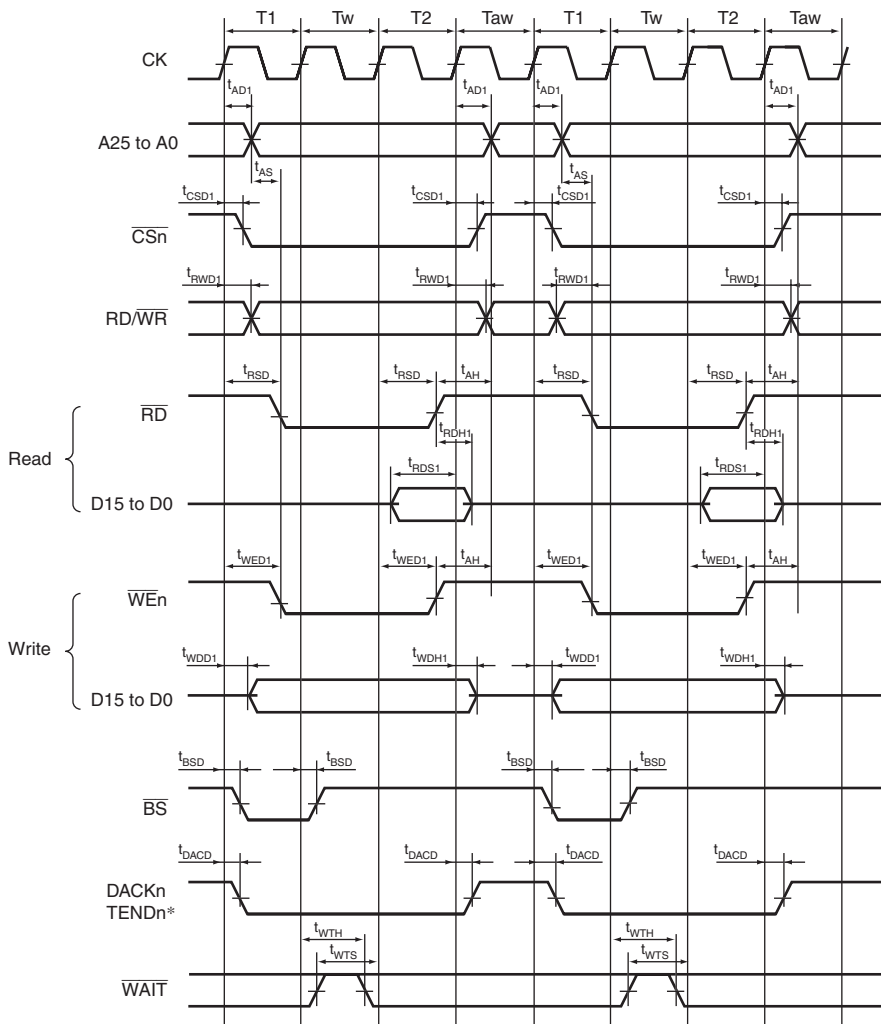
Figure 31.14 Basic Bus Timing for Normal Space (One Software Wait Cycle, External Wait Cycle Valid (WM Bit = 0), No Idle Cycle)
