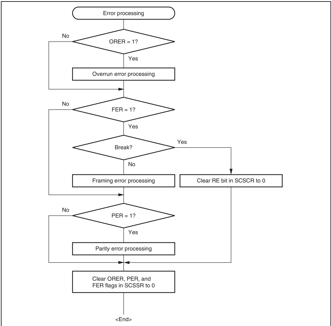
Figure 16.6 Sample Flowchart for Receiving Serial Data (2)
