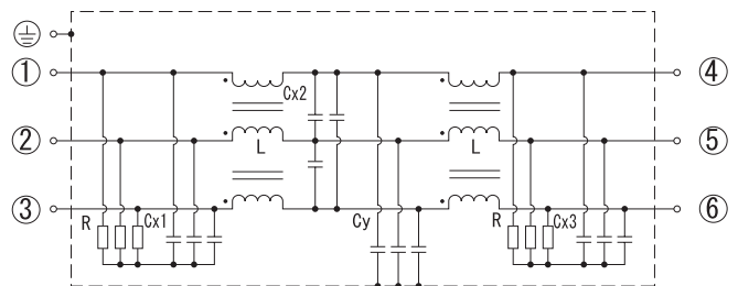
Circuit
