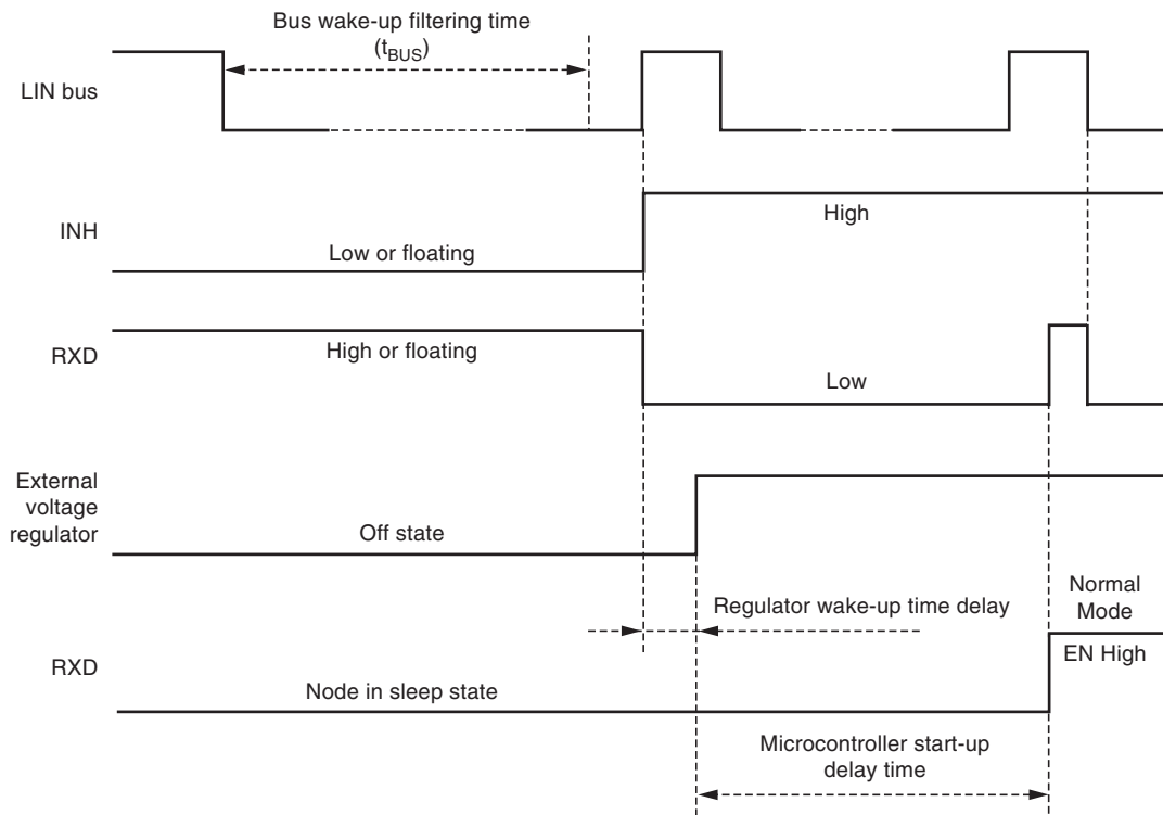
Figure 3-2. LIN Wake-up Waveform Diagram
