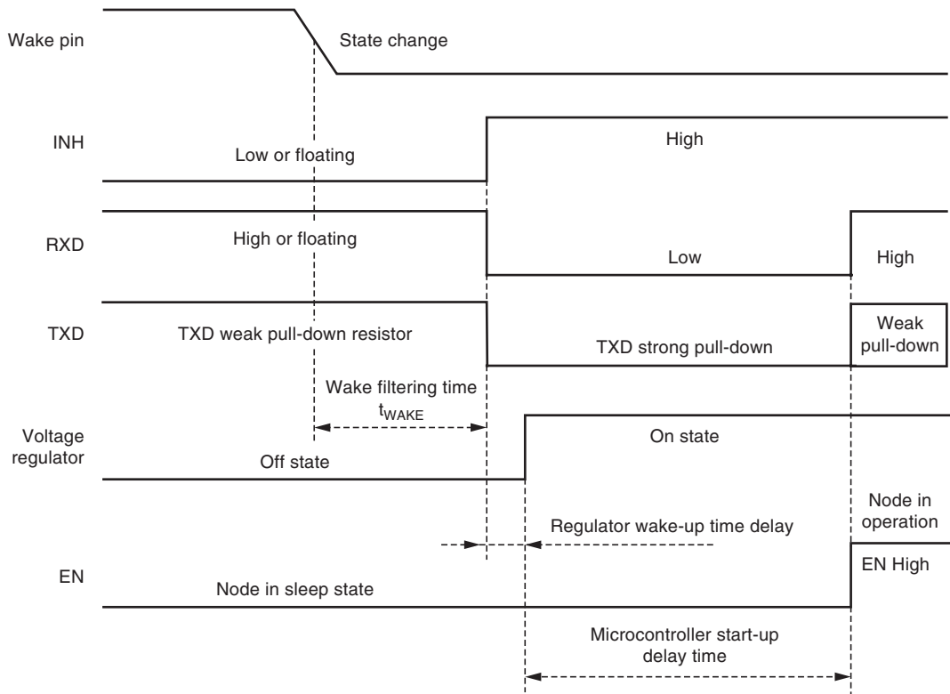
Figure 3-3. Wake-up from Wake-up Switch
