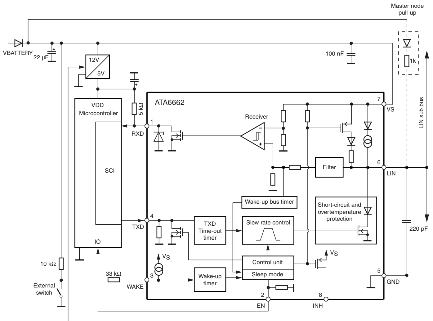
Figure 6-2. Application Circuit
