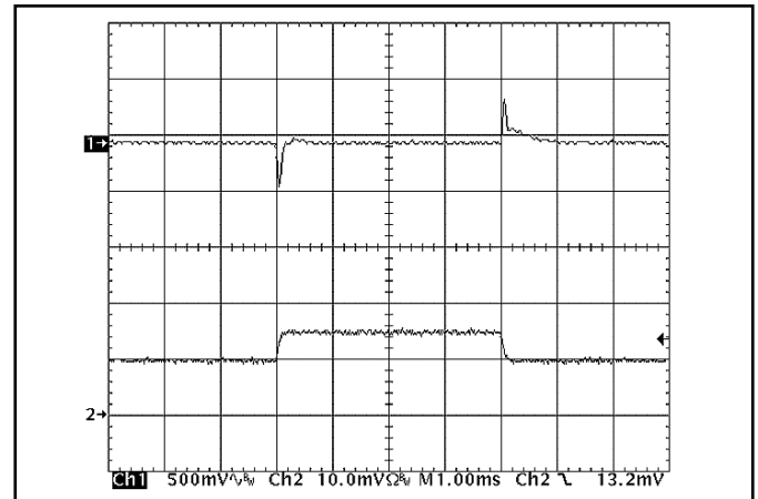
Figure 10: Output voltage response to step-change in load current (50%-75%-50% of Iout(max); dI/dt = 5A/\mu s ). Load cap: 480 \mu F , 15 m \Omega ESR tantalum cap and 1 \mu F ceramic cap. Top trace: Vout (500mV/div), Bottom trace: Iout (5A/div).
