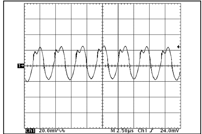
Figure 14: Output voltage ripple at nominal input voltage and rated load current (20 mV/div). Load capacitance: 1\ \mu\text{F} ceramic capacitor and 15\ \mu\text{F} tantalum capacitor. Bandwidth: 20 MHz. See Figure 11.
