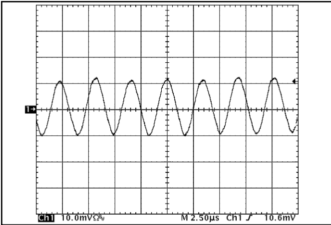
Figure 13: Input reflected ripple current, i_v , through a 10\ \mu\text{H} source inductor at nominal input voltage and rated load current (10 mA/div). See Figure 11.
