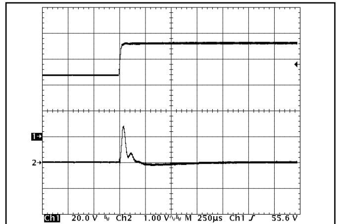
Figure 16: Output voltage response to step-change in input voltage (1000V/ms). Ch1: V_{in} (20V/div), Ch2: V_{out} (1V/div).
