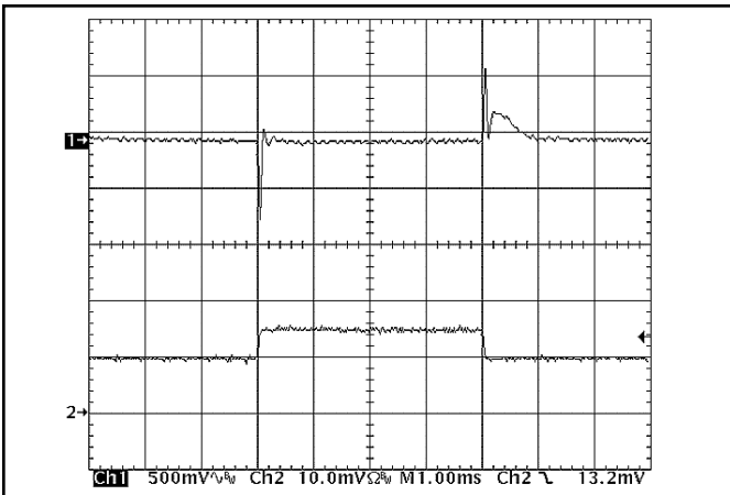
Figure 9: Output voltage response to step-change in load current (50%-75%-50% of Iout(max); dI/dt = 0.1A/\mu s ). Load cap: 15 \mu F , 450 m \Omega ESR tantalum cap and 1 \mu F ceramic cap. Top trace: Vout (500mV/div), Bottom trace: Iout (5A/div).
