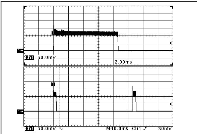
Figure 15: Load current (5A/div) as a function of time when the converter attempts to turn on into a 10\ \text{m}\Omega short circuit. Top trace (2ms/div) is an expansion of the on-time portion of the bottom trace.
