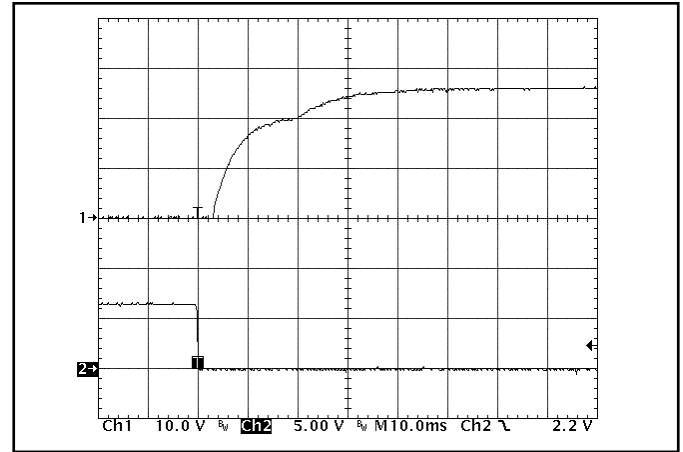
Figure 8: Turn-on transient at zero load (10 ms/div). Top Trace: Vout (10V/div). Bottom Trace: ON/OFF input (5V/div).
