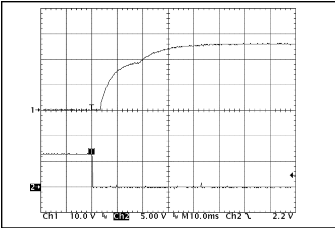
Figure 7: Turn-on transient at full load (resistive load) (10 ms/div). Input voltage pre-applied. Top Trace: Vout (10V/div). Bottom Trace: ON/OFF input (5V/div).
