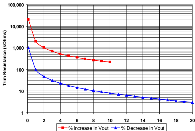
Figure C: Trim Graph for 26Vout module
