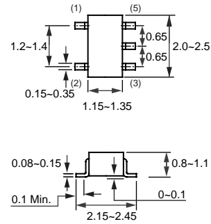
SC-88A/SOT353
