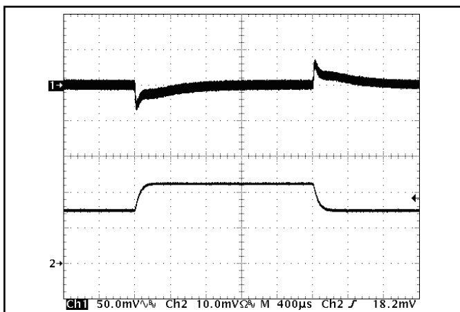
Figure 11: Output voltage response to step-change in load current (50%-75%-50% of I out (max); di/dt = 0.1A/μs). Load cap: 10uF, 100 mΩ ESR tantalum cap and 1uF ceramic cap. Ch 1: V out (50mV/div), Ch 2: I out (10A/div).
