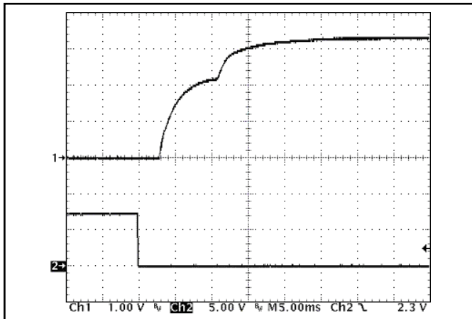
Figure 9: Turn-on transient at full load (resistive load) (5 ms/div). Load cap: 10uF, 100 mΩ ESR tantalum capacitor and 1uF ceramic capacitor. Input voltage pre-applied. Ch 1: V out (1V/div), Ch 2: ON/OFF input (5V/div).
