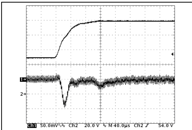
Figure 17: Output voltage response to step-change in input voltage (50V to 100V in 100µs), at 15A load current. Load cap: 15\ \mu\text{F} 100\ \text{m}\Omega ESR tantalum capacitor and 1\ \mu\text{F} ceramic cap. Ch 1: V_{out} (50mV/div), Ch 2: V_{in} (20V/div).
