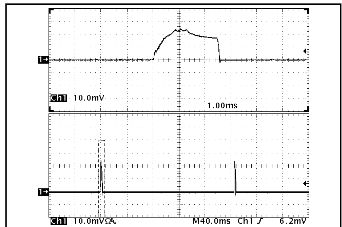
Figure 18: Load current (20A/div) as a function of time when the converter attempts to turn on into a 15\ \text{m}\Omega short circuit. Top trace (1ms/div) is an expansion of the on-time portion of the bottom trace (40ms/div).
