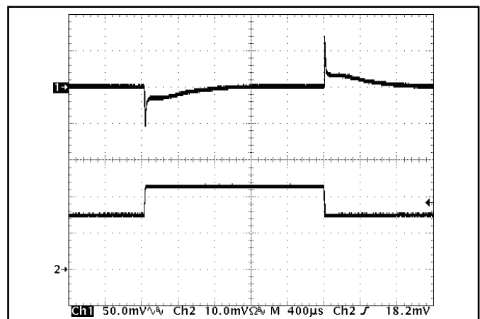
Figure 12: Output voltage response to step-change in load current (50%-75%-50% of I out (max); di/dt = 1A/μs). Load cap: 470uF, 30 mΩ ESR tantalum cap and 1uF ceramic cap. Ch 1: V out (50mV/div), Ch 2: I out (10A/div).
