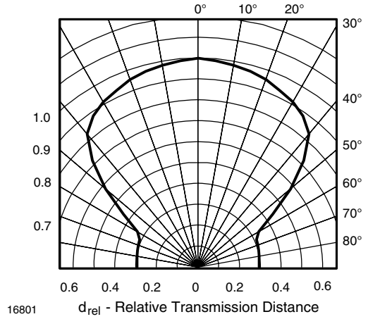
Fig. 12 - Directivity
