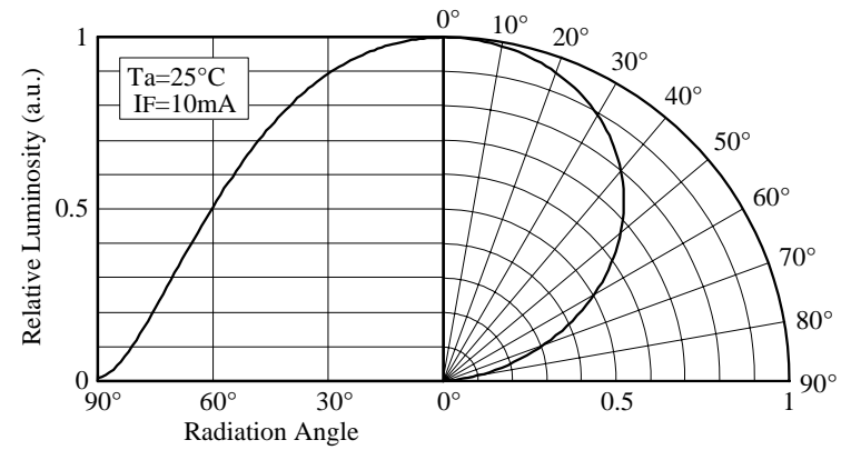
■ Directivity (NECG426B)
