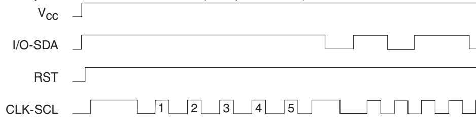
Figure 11. Synchronous 2-wire Protocol (Gemplus Patent)
