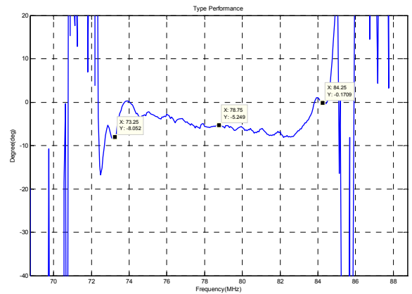
Phase Linearity(f0±5.5MHz)
