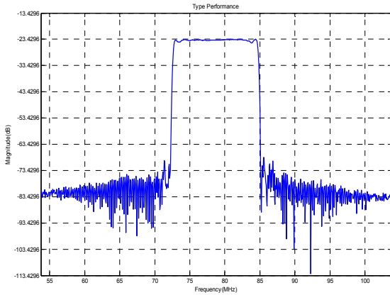
Frequency Respond
