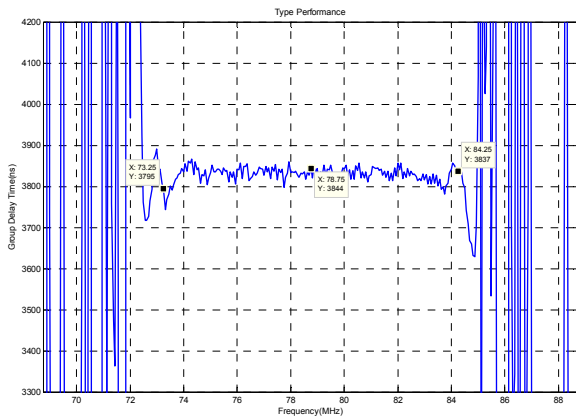
Group Delay Variation(f0±5.5MHz)
