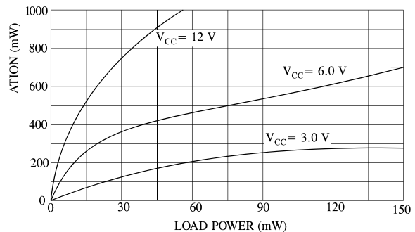
Figure 2. DEVICE DISSIPATION 8.0 Ω LOAD
