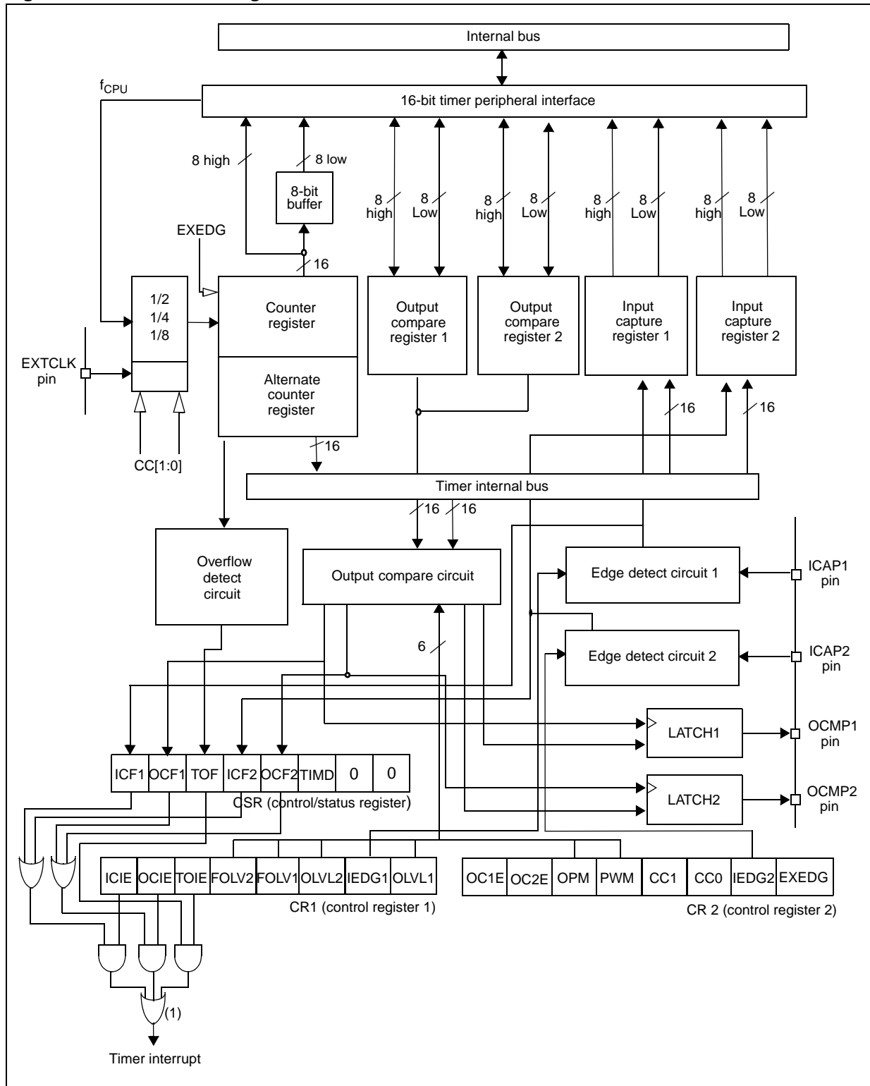
Figure 55. Timer block diagram
