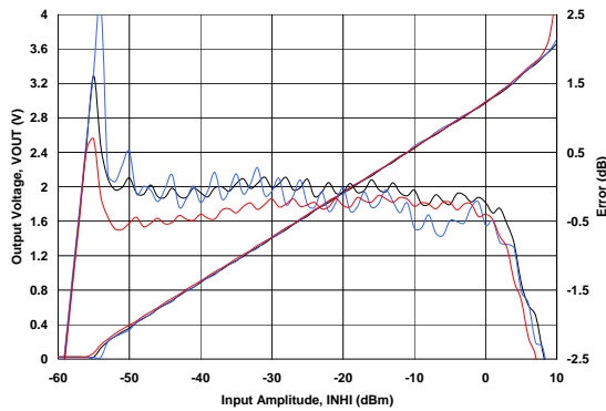
Figure 4. V_{OUT} Voltage and Log Conformance vs. Input Amplitude at 900 MHz, Typical Device, T_{CM1} = 0.48\text{ V} , T_{CM2} = 1.2\text{ V} , Sine Wave, -40^\circ\text{C} , 25^\circ\text{C} , 85^\circ\text{C}
