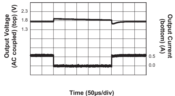
Load Transient (1mA to 600mA; V_{IN} = 3.6V ; V_{OUT} = 1.8V ; C_{OUT} = 4.7µF ; C_{FF} = 100pF )
