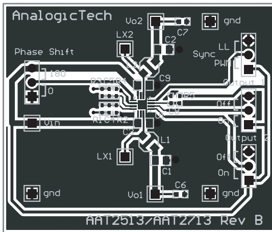
Figure 3: AAT2713 Evaluation Board Top Side.
