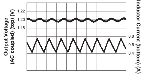
Time (500ns/div)
