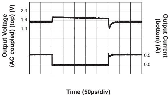
Load Transient (1mA to 600mA; V_{IN} = 3.6V ; V_{OUT} = 1.8V ; C_{OUT} = 4.7µF ; C_{FF} Open)
