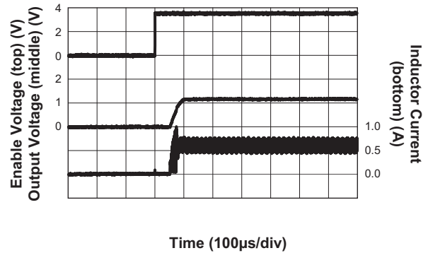
Soft Start ( V_{IN} = 3.6V ; V_{OUT} = 1.2V ; I_{OUT} = 600mA )
