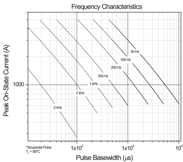
Fig. 9 - Frequency Characteristics
