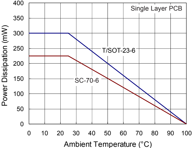
Figure 1. De-rating Curves
