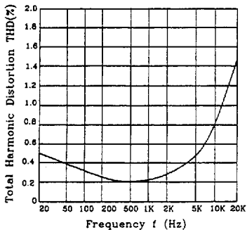
Total Harmonic Distortion vs. Frequency (V + =6V, R L =8Ω, P o =125mW, A v =26dB)
