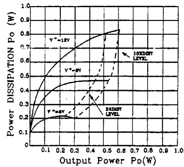
Power Dissipation vs. Output Power (RL=8Ω)
