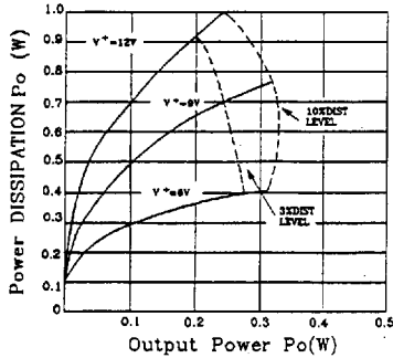
Power Dissipation vs. Output Power (RL=4Ω)
