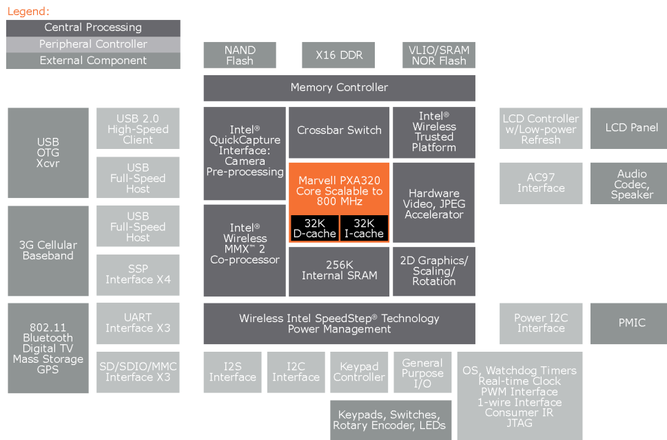
PXA320 Processor Block Diagram
