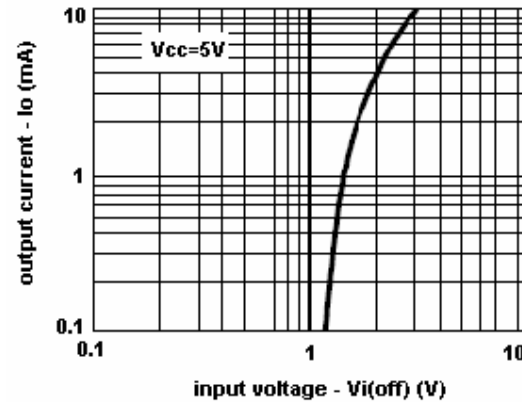
output current vs input voltage (off)
