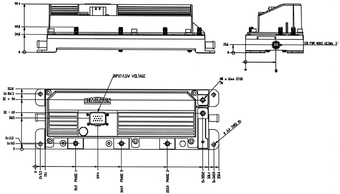
SKAI 7001MD075 1452 W: General dimensions
