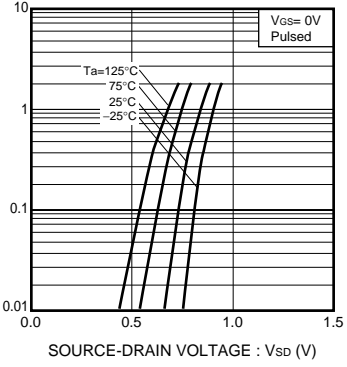
Fig.6 Source Current vs. Source-Drain Voltage
