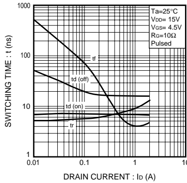
Fig.2 Switching Characteristics
