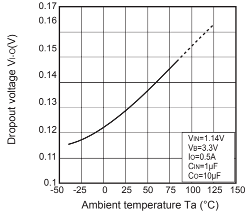
Fig.21 Dropout Voltage vs. Ambient Temperature (PQ012GN01ZPH)
