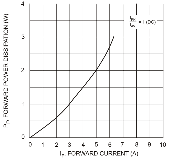
Fig. 6 Forward Power Dissipation
