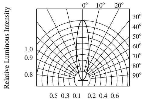
FIG.6 RADIATION DIAGRAM
