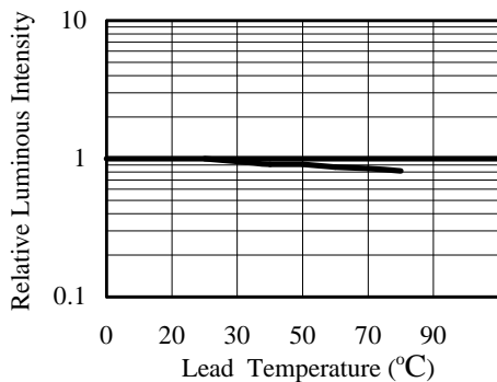
FIG.5 LUMINOUS INTENSITY VS. LEAD TEMPERATURE
