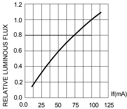
FIG.2 FORWARD CURRENT.
