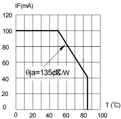
FIG.4 MAXIMUM FORWARD DC CURRENT VS TEMPERATURE. DERATING BASED ON T_{jmax}=110^\circ\text{C}
