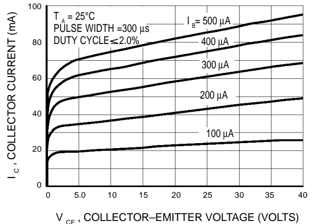
Figure 10. Collector Characteristics
