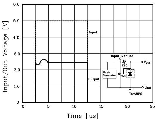
Fig. 8 Pulse response
