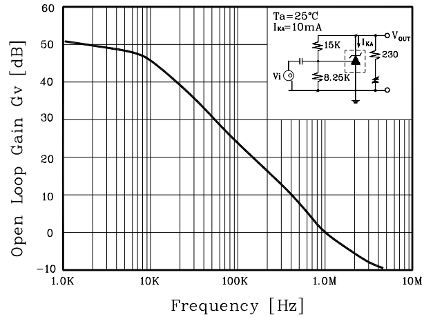
Fig. 7 G_v vs. frequency
