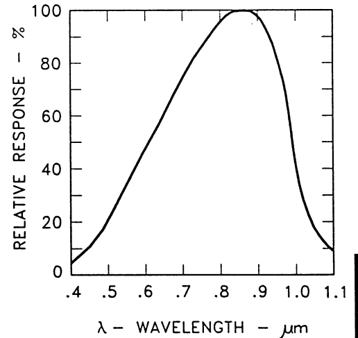
SPECTRAL RESPONSIVITY
