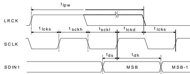
Figure 2. TDM Serial Audio Interface Timing
