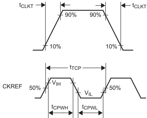
Figure 17. LVC MOS Clock Parameters
