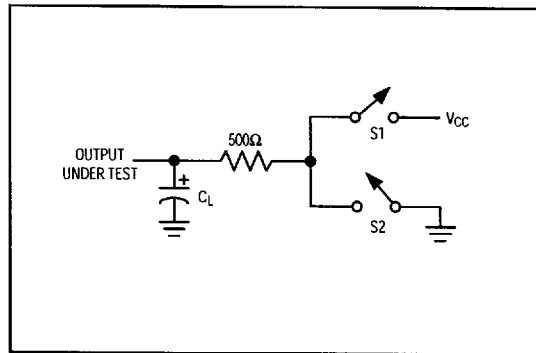
Figure 11. Driver Timing Test Load
