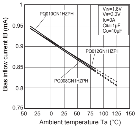
Fig.10 Bias Inflow Current vs. Ambient Temperature
