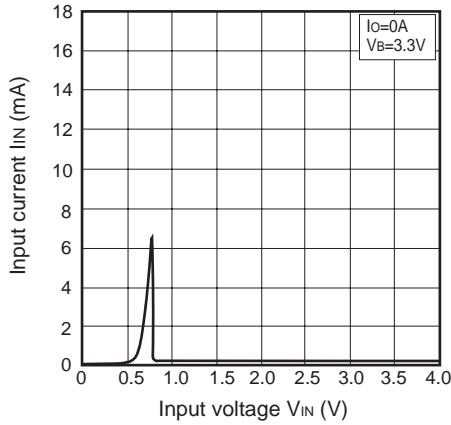
Fig.20 Input Current vs. Input Voltage (PQ008GN1HZPH)
