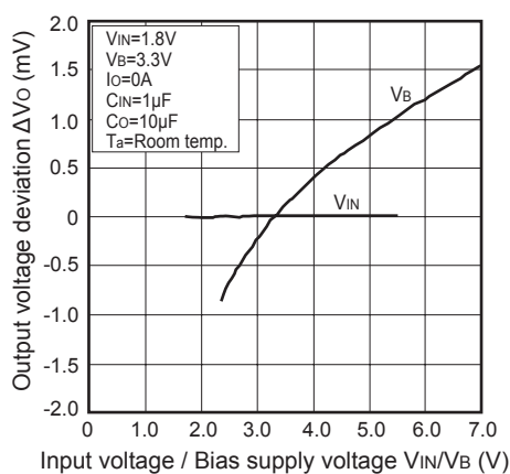
Fig.17 Output Voltage Deviation vs. Input Voltage / Bias Supply Voltage (PQ008GN1HZPH)
