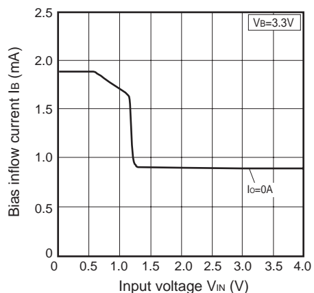
Fig.25 Bias Inflow Current vs. Input Voltage (PQ012GN1HZPH)
