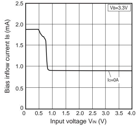
Fig.23 Bias Inflow Current vs. Input Voltage (PQ008GN1HZPH)
