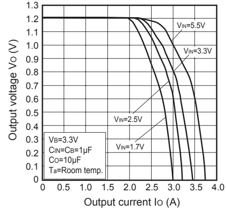
Fig.5 Overcurrent Protection Characteristics (PQ012GN1HZPH)
