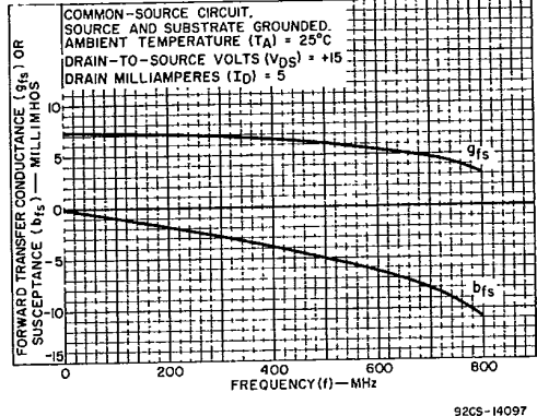
Fig. 12 - Forward Transadmittance (Y fs ) Components
