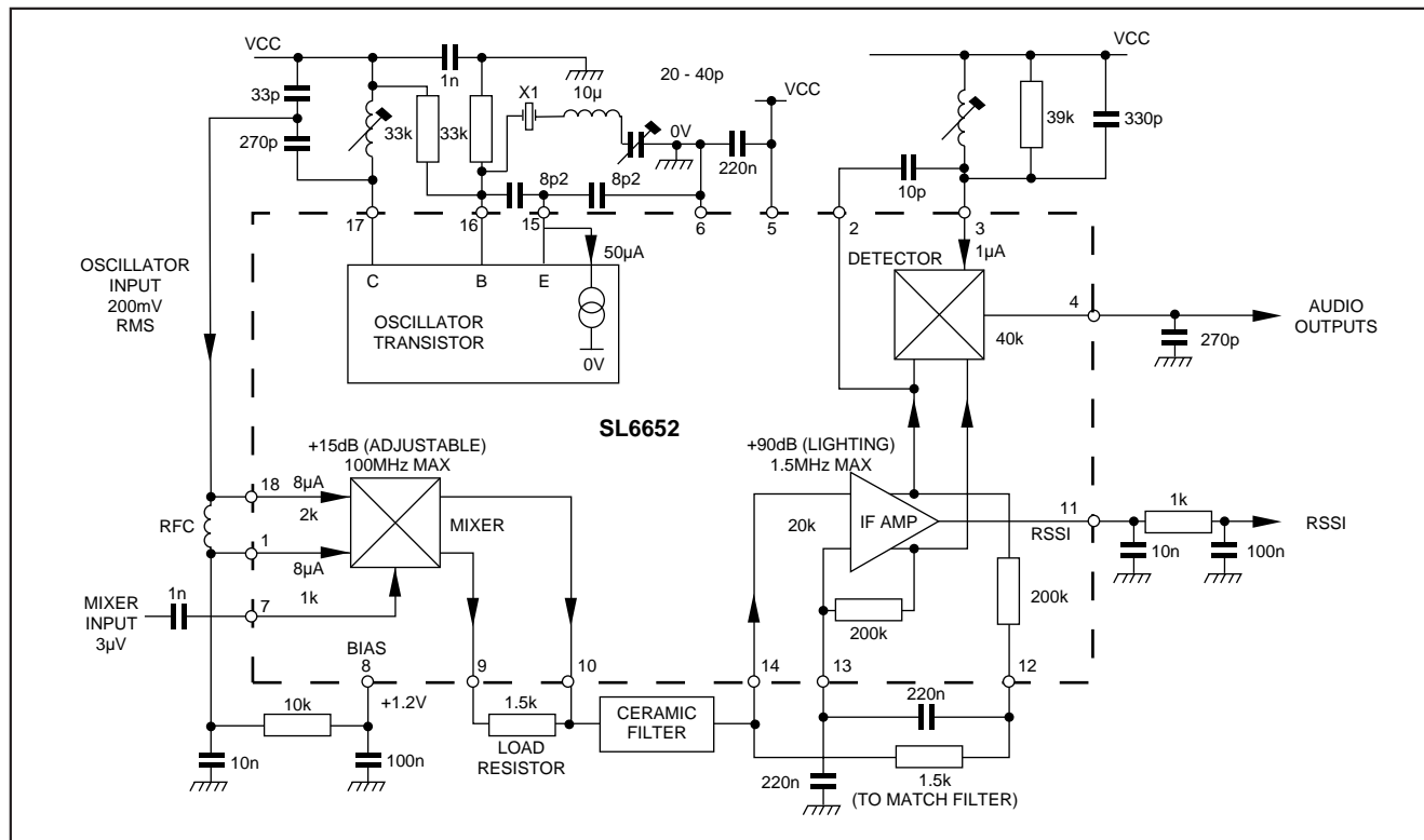
Fig. 2 block diagram
